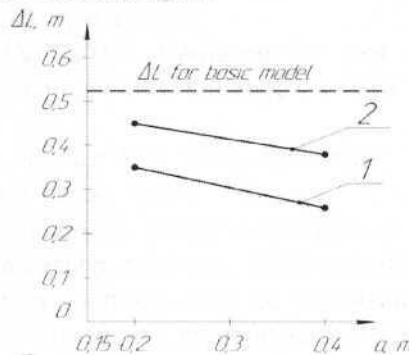
Fig. 8 - Dependence of the length of the stem \Delta L with basket reaching a threshing wheel on the length of the rotor a and the angle of its inclination to the surface of the soil
