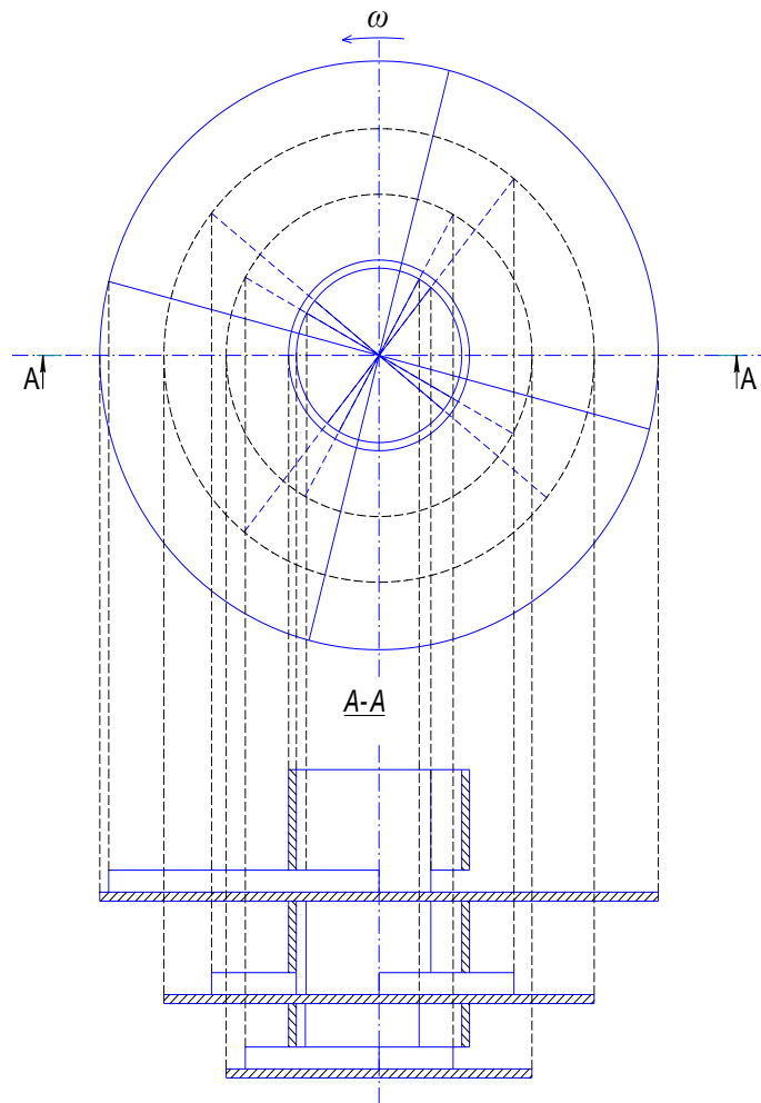
Fig. 3 – Design of spreader's construction
