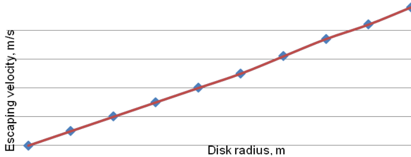
Fig. 5 - The dependence of granule escaping velocity on the disk radius
