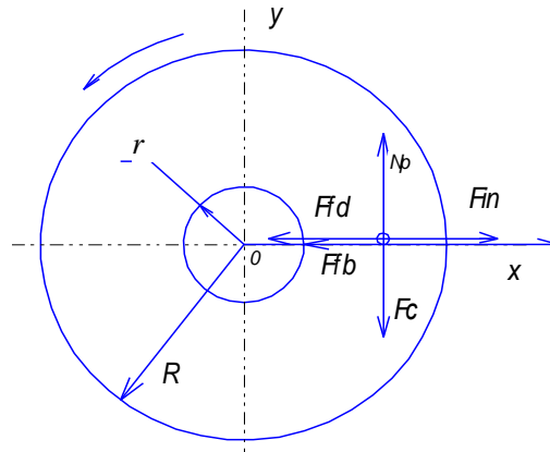
Fig. 4 - Scheme of forces distribution that influences the granule during disk rotation
